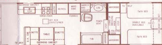
35' Center Bath - Dry Wt. 7500 lbs. - Hitch Wt. 1750 lbs. - Overall Length 32'6"
