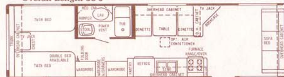
33' Center Bath Dinette - Dry Wt. 6900 lbs. - Hitch Wt. 700 lbs. - Overall Length 33'5"
