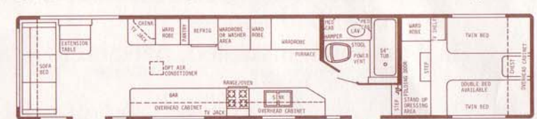
40' Front Bath Doorside Kitchen - Dry Wt. 9300 lbs. - Hitch Wt. 1650 lbs. - Overall Length 39'6"
