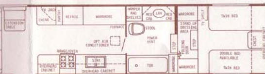
35' Front Bath Doorside Kitchen - Dry Wt. 7500 lbs. - Hitch Wt. 1750 lbs. - Overall Length 32'6"
