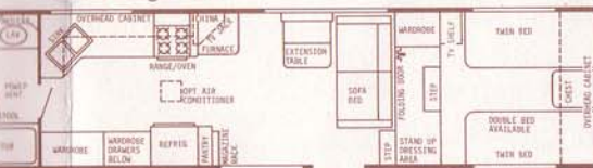
35' Rear Bath - Dry Wt. 7500 lbs. - Hitch Wt. 1750 lbs. - Overall Length 32'6"
