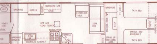
35' Walk-Thru Front Bath - Dry Wt. 7500 lbs. - Hitch Wt. 1750 lbs. - Overall Length 32'6"
