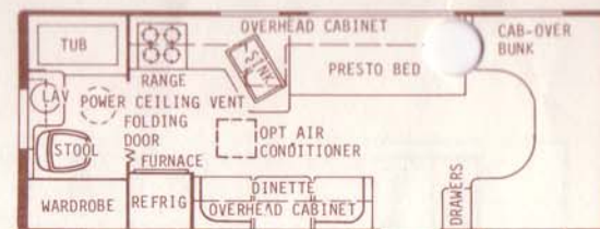
23RB - Dry Wt. 9600 lbs. - Overall length 24'4"
