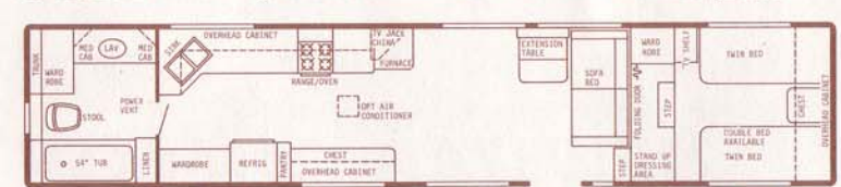
40' Rear Bath Plan #2 - Dry Wt. 9300 lbs. - Hitch Wt. 1650 lbs. - Overall Length 39'6"
