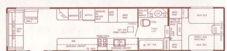
40' Walk-Thru Front Bath - Dry Wt. 9300 lbs. - Hitch Wt. 1650 lbs. - Overall Length 39'6"
