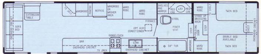
40' Walk-Thru Front Bath - Dry Wt. 9300 lbs. - Hitch Wt. 1650 lbs. - Overall Length 39'6"
