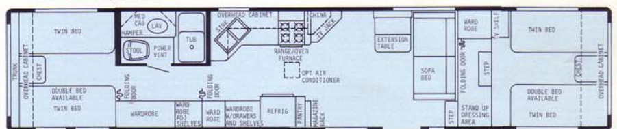
40' Center Bath - Dry Wt. 9300 lbs. - Hitch Wt. 1650 lbs. - Overall Length 39'6"
