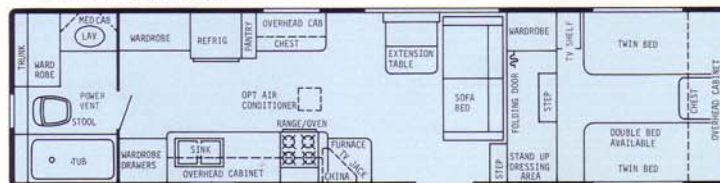
32' Rear Bath Doorside Kitchen - Dry Wt. 7500 lbs. - Hitch Wt. 1650 lbs. - Overall Length 32'6"
