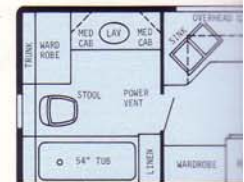
35' Rear Bath Plan #2 - Dry Wt. 8500 lbs. - Overall Length 35'6"
