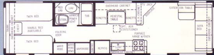
35' Center Bath Dinette - Dry Wt. 7000 lbs. - Hitch Wt. 700 lbs. - Overall Length 34'6"
