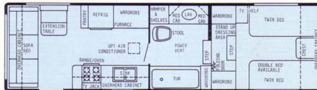
28' Walk-Thru Front Bath - Dry Wt. 6600 lbs. - Hitch Wt. 1650 lbs. - Overall Length 28'8"
