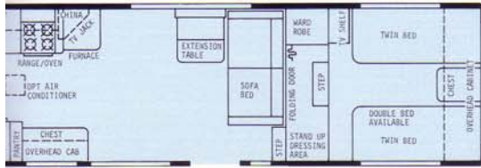
40' Rear Bath Plan #2 - Dry Wt. 8500 lbs. - Hitch Wt. 1650 lbs.
