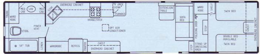
40' Rear Bath Plan #2 - Dry Wt. 9300 lbs. - Hitch Wt. 1750 lbs. - Overall Length 39'6"
