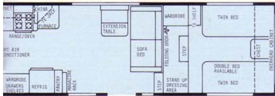
40' Rear Bath Plan #1 - Dry Wt. 8500 lbs. - Hitch Wt. 1650 lbs.
