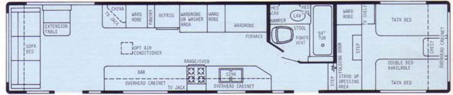
40' Front Bath Doorside Kitchen - Dry Wt. 9300 lbs. - Hitch Wt. 1650 lbs. - Overall Length 39'6"
