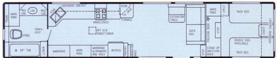
40' Rear Bath Plan #1 - Dry Wt. 9300 lbs. - Hitch Wt. 1750 lbs. - Overall Length 39'6"
